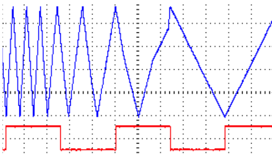
Figure 1a: Changing Div/Mult gradually (slow knob movement) Slope of envelope tracks the Div/Mult amount until the knob stops turning (about half-way across the figure), at which point it re-syncs to the ping clock.
