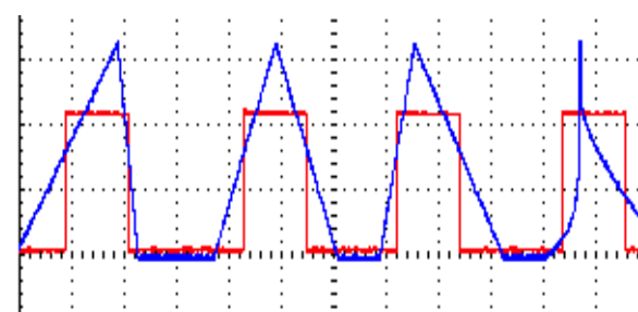
Figure 12a: Half-Rise Gate HR goes high 1/2 through time of Rise (regardless of curve/skew/shape).
