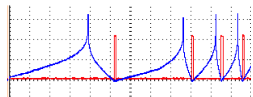
Figure 11b: EOF Trigger output Width of trigger is 4ms
