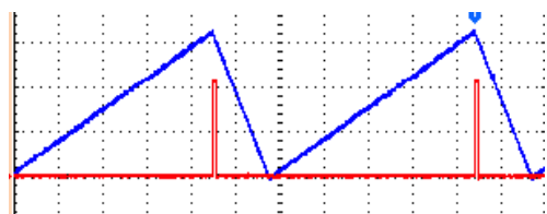
Figure 10b: EOR Trigger output Width of trigger is 4ms
