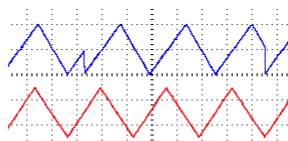
Figure 3c: QNT trigger used to re-phase Blue channel (top) and Red channel (bottom) both set to /4 , pinged by same clock. Blue is re-phased twice with QNT trigger. Envelopes start in-phase, then Blue lags by 90^\circ , then they are re-phased back together.
