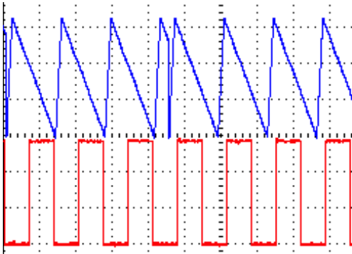
Figure 13a: Async mode (re-triggering) Envelope starts at the same point on the ping clock: for the first 3 clocks it's approximately the falling edge of the ping. About half-way through the figure, another async trigger is given and the reset point becomes a little bit before the rising edge.
